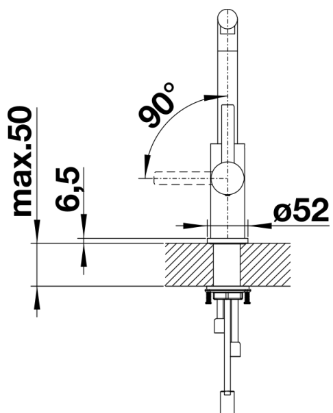
Side view hand gear 2D
